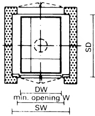
① Plan view of shaft
